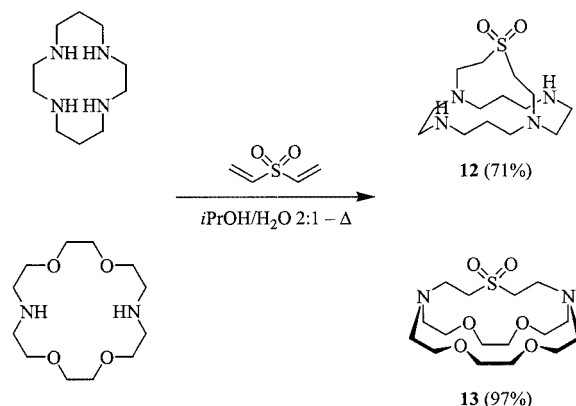
Scheme 7. Cryptands from commercially available macrocycles
