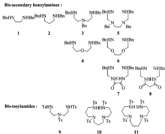
Figure 1. Utilized bis-secondary amines and tosylamides
