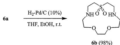
Scheme 6. Cleavage of benzyl groups in an S,S -dioxothia macrocycle
