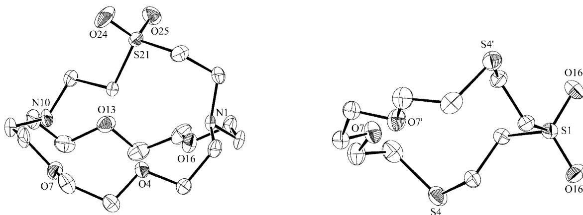
Figure 5. ORTEP drawings of the crystal structures of compounds 13 and 16a
