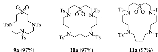
Figure 3. New S,S -dioxothia macrocycles from divinyl sulfone and bis(sulfonamides)
