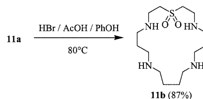
Scheme 8. Cleavage of tosyl groups
