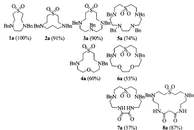
Figure 2. New S,S -dioxothia macrocycles from divinyl sulfone and bis-secondary amines
