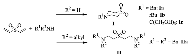
Scheme 3. Aza-Michael addition of various amines to divinyl sulfone
