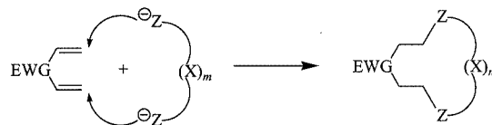
Scheme 2. A new strategy to obtain macrocycles from bis-Michael acceptors
