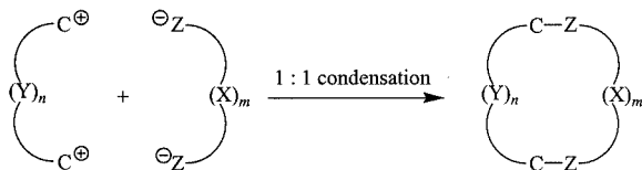
Scheme 1. Construction of a macrocyclic compound from two fragments
