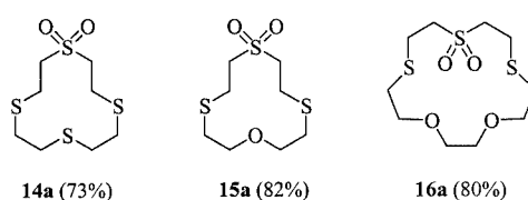
Figure 4. New thia and oxathia macrocyclic sulfones from divinyl sulfone and bis(thiols)
