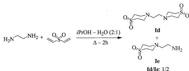
Scheme 4. Aza-Michael addition of ethylenediamine to divinyl sulfone
